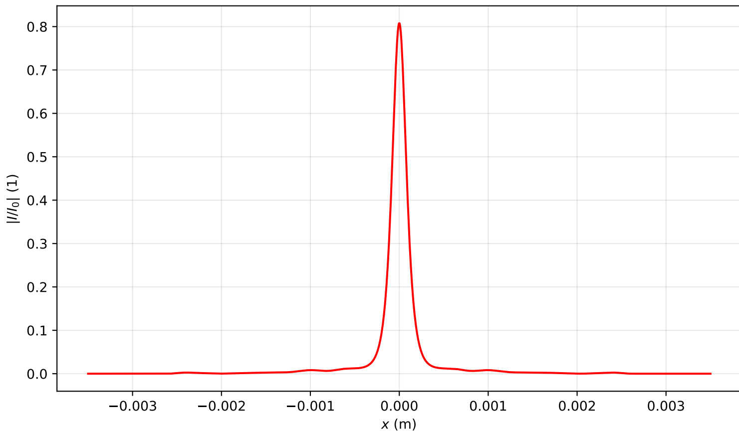
Intensity profile I(x, y = 0, z = 3.344)/I_0 , P_{in}=13.0P_{cr} , artificial time
