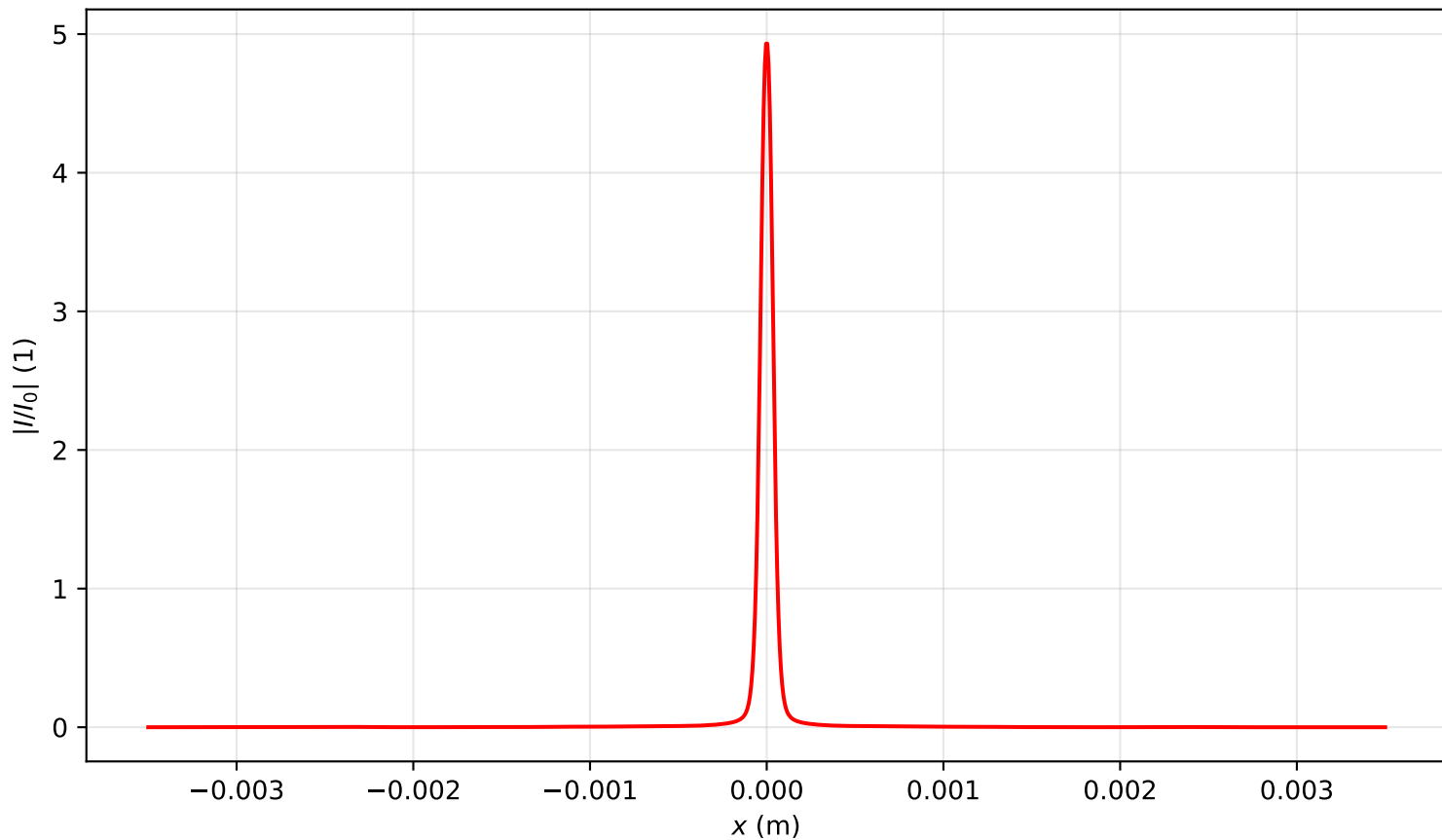
Intensity profile I(x, y = 0, z = 3.503)/I_0 , P_{in}=13.0P_{cr} , artificial time
