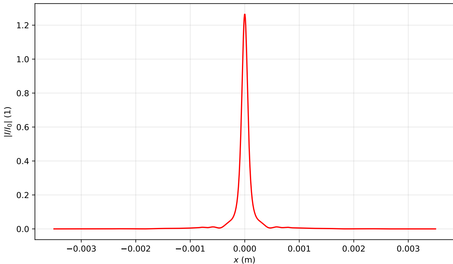
Intensity profile I(x, y = 0, z = 3.662)/I_0 , P_{in}=13.0P_{cr} , artificial time
