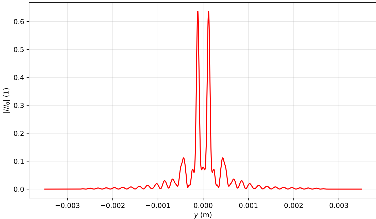
Intensity profile I(x=0, y, z=0.159)/I_0 , P_{in}=13.0P_{cr} , artificial time
