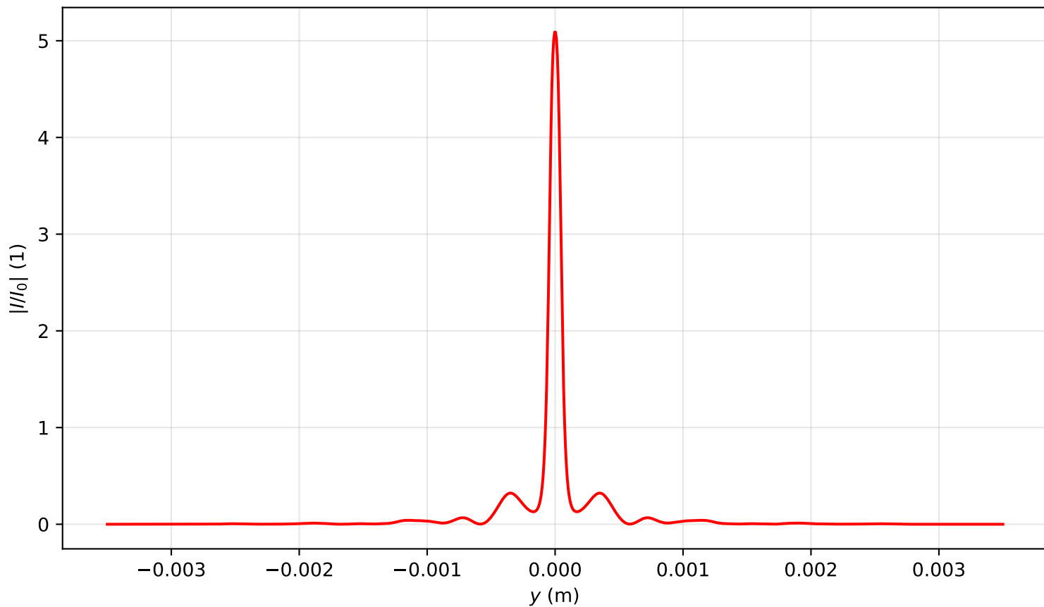
Intensity profile I(x=0, y, z=0.478)/I_0 , P_{in}=13.0P_{cr} , artificial time
