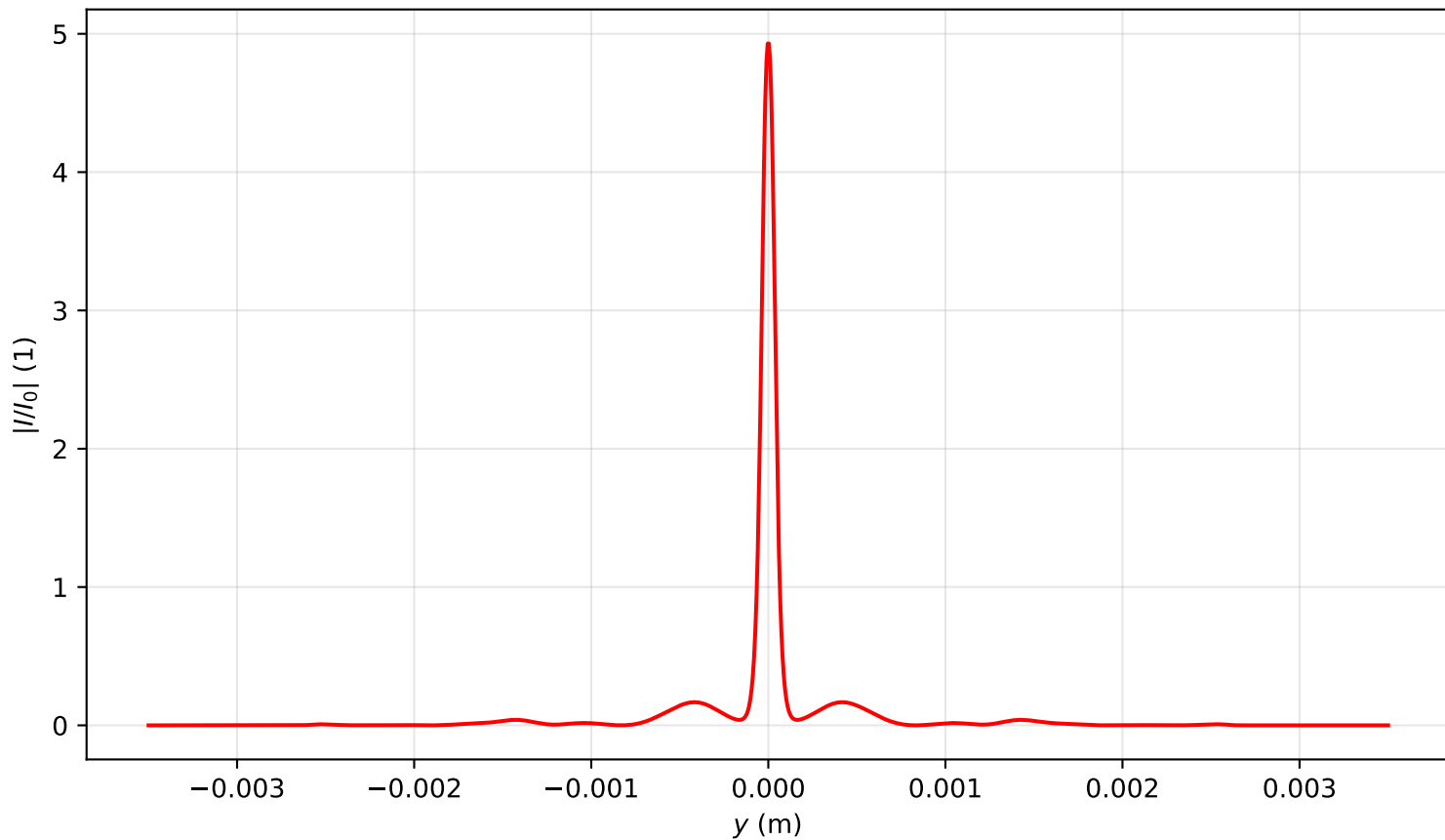
Intensity profile I(x=0, y, z=0.637)/I_0 , P_{in}=13.0P_{cr} , artificial time
