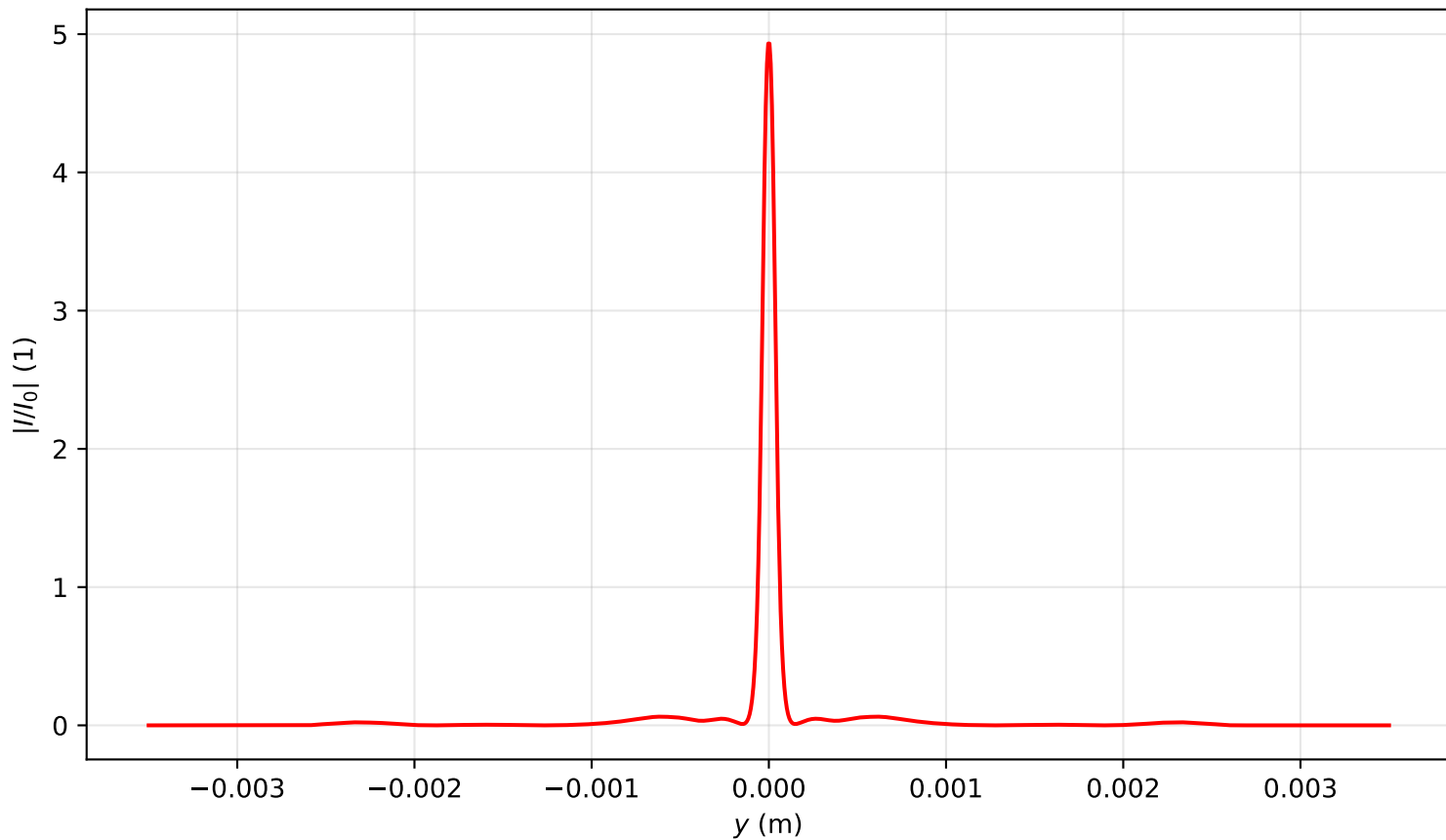
Intensity profile I(x=0, y, z=0.955)/I_0 , P_{in}=13.0P_{cr} , artificial time
