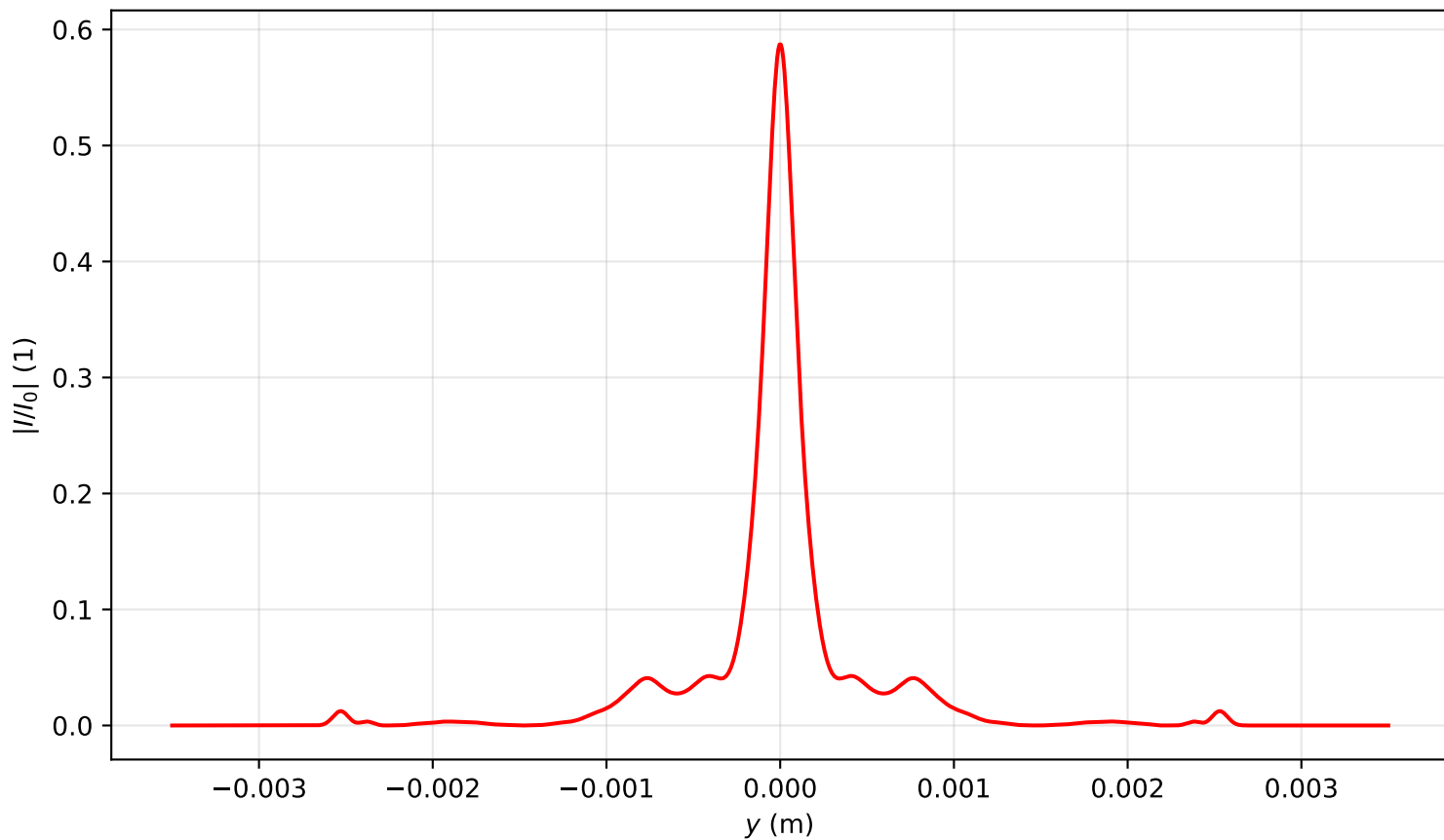
Intensity profile I(x=0, y, z=1.115)/I_0 , P_{in}=13.0P_{cr} , artificial time
