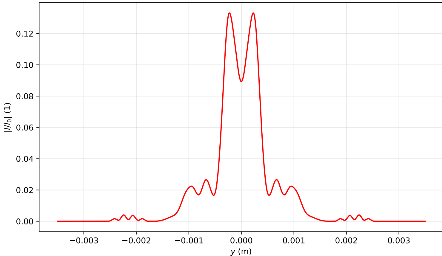
Intensity profile I(x=0, y, z=1.274)/I_0 , P_{in}=13.0P_{cr} , artificial time
