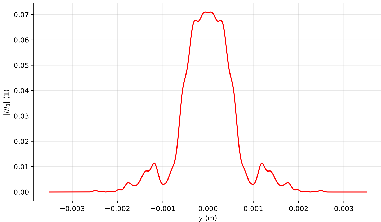
Intensity profile I(x=0, y, z=1.751)/I_0 , P_{in}=13.0\text{Pcr} , artificial time
