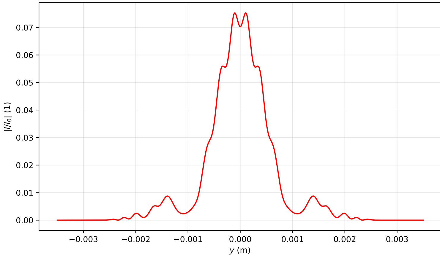
Intensity profile I(x=0, y, z=1.911)/I_0 , P_{in}=13.0P_{cr} , artificial time
