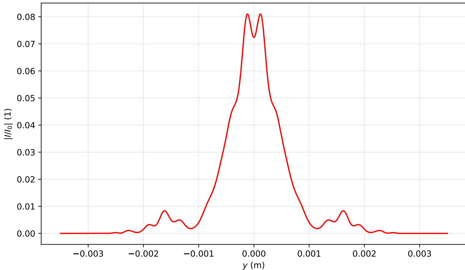
Intensity profile I(x = 0, y, z = 2.070)/I_0 , P_{in}=13.0P_{cr} , artificial time
