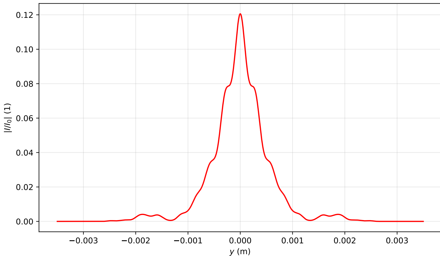
Intensity profile I(x=0, y, z=2.229)/I_0 , P_{in}=13.0P_{cr} , artificial time
