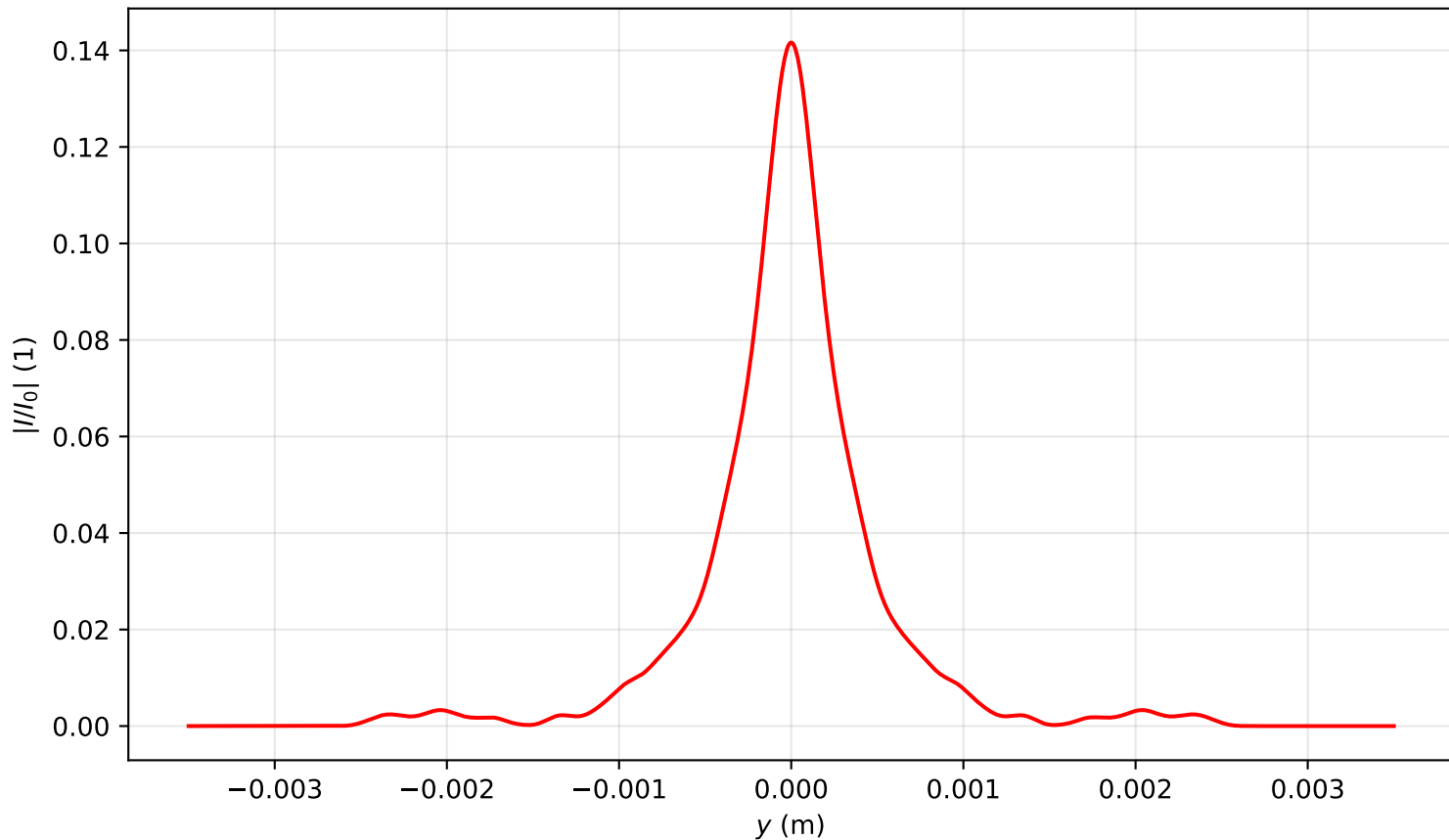
Intensity profile I(x=0, y, z=2.548)/I_0 , P_{in}=13.0P_{cr} , artificial time
