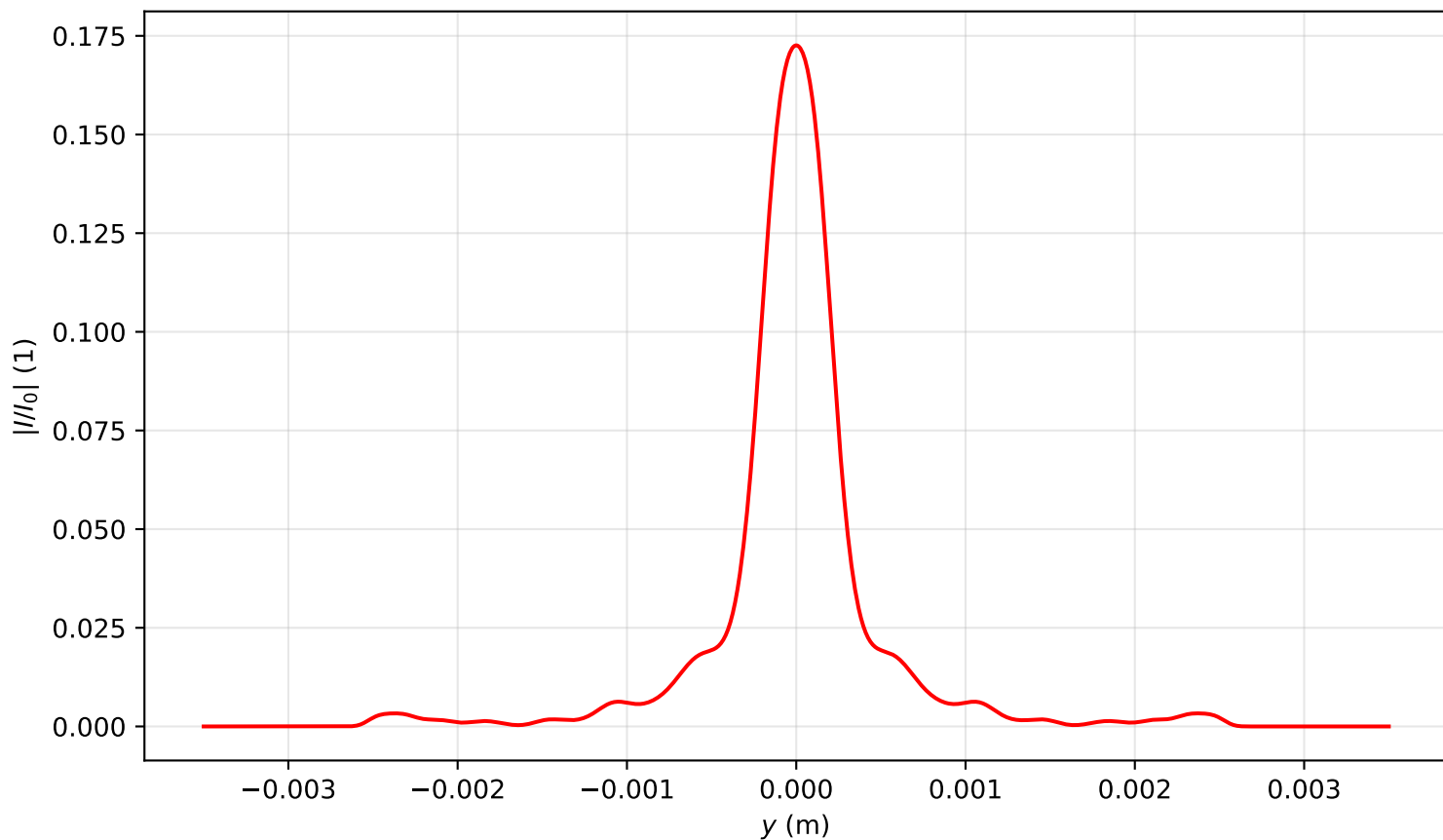
Intensity profile I(x=0, y, z=2.866)/I_0 , P_{in}=13.0\text{Pcr} , artificial time
