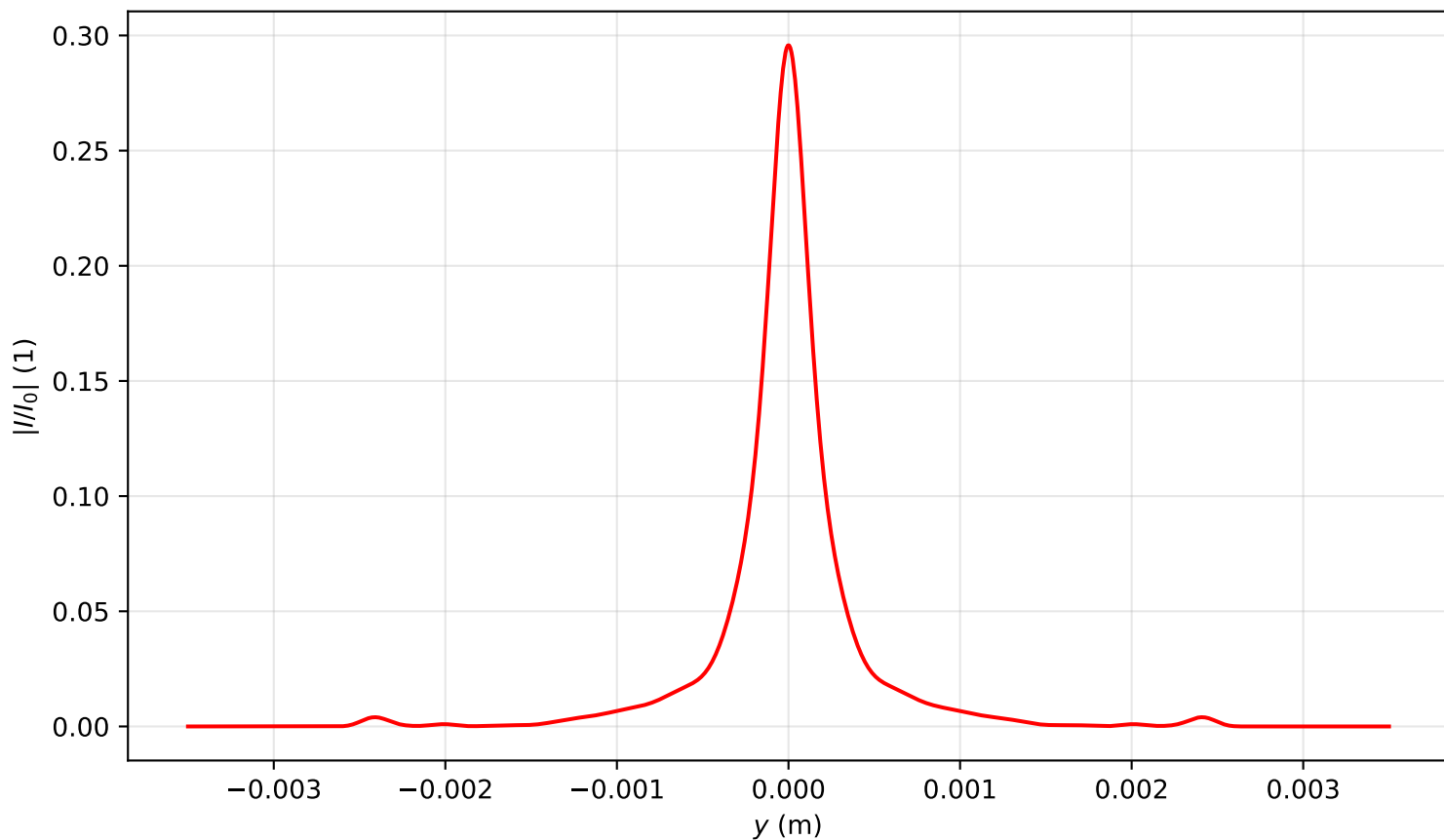
Intensity profile I(x=0, y, z=3.025)/I_0 , P_{in}=13.0P_{cr} , artificial time
