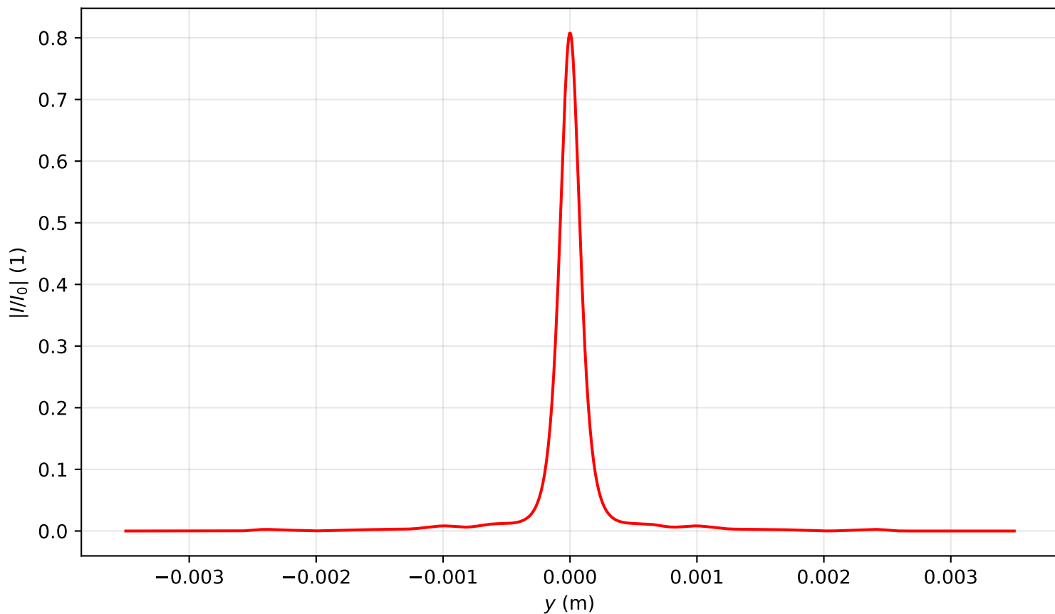
Intensity profile I(x=0, y, z=3.344)/I_0 , P_{in}=13.0P_{cr} , artificial time
