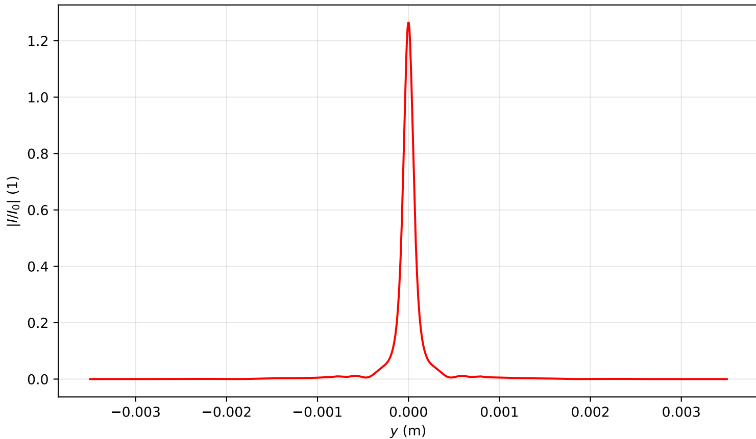
Intensity profile I(x=0, y, z=3.662)/I_0 , P_{in}=13.0P_{cr} , artificial time
