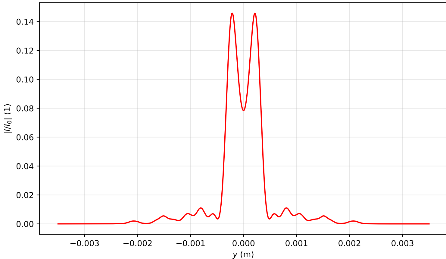
Intensity profile I(x=0, y, z=3.821)/I_0 , P_{in}=13.0P_{cr} , artificial time
