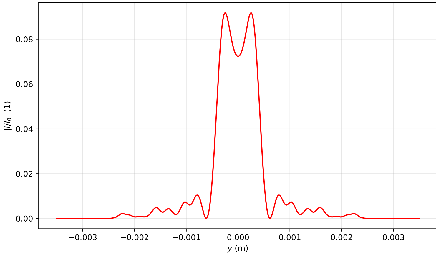
Intensity profile I(x=0, y, z=3.981)/I_0 , P_{in}=13.0\text{Pcr} , artificial time
