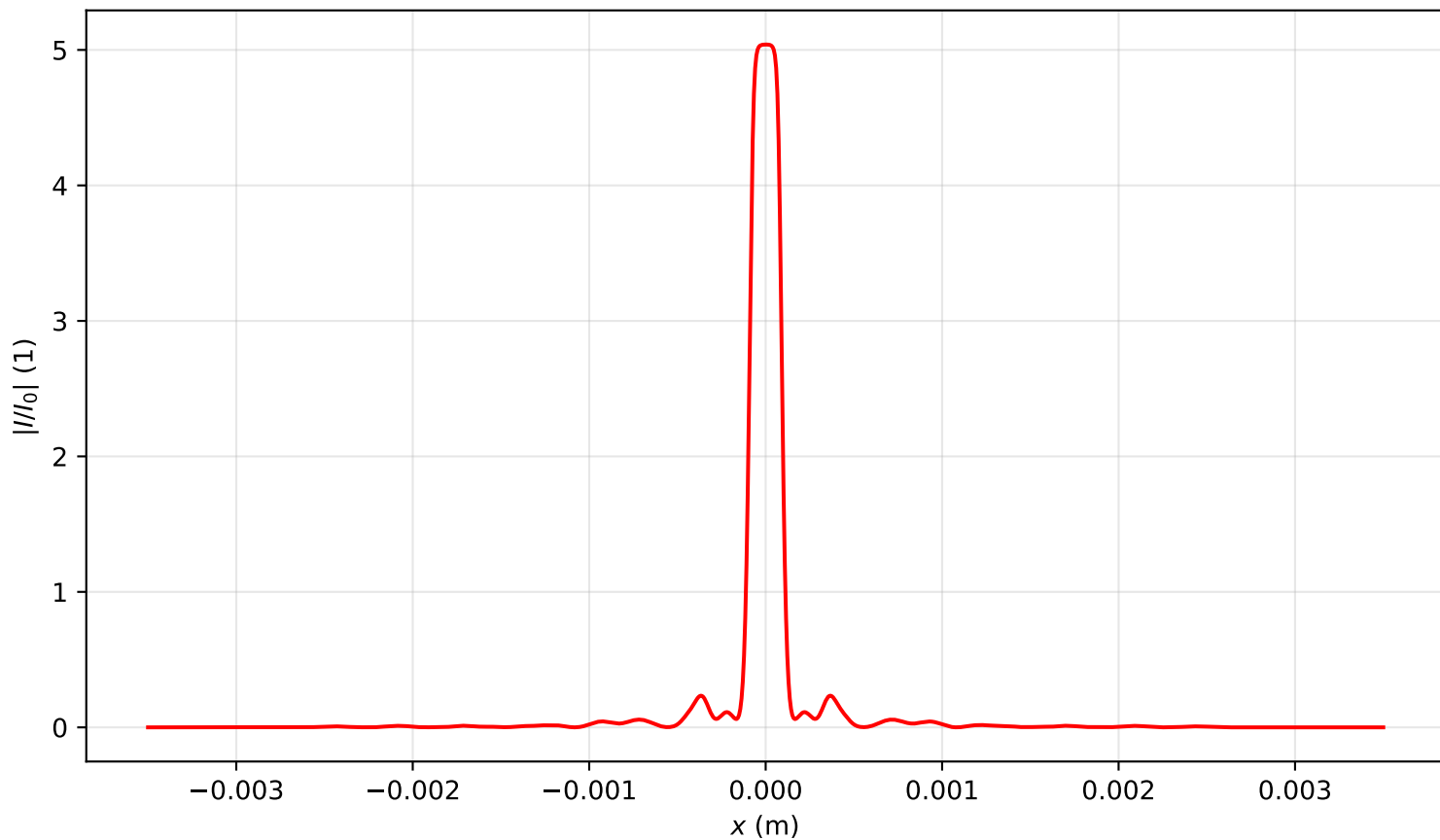
Intensity profile I(x, y = 0, z = 0.318)/I_0 , P_{in}=14.0P_{cr} , artificial time
