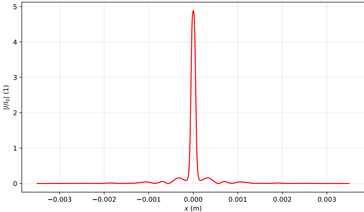
Intensity profile I(x, y = 0, z = 0.478)/I_0 , P_{in}=14.0P_{cr} , artificial time
