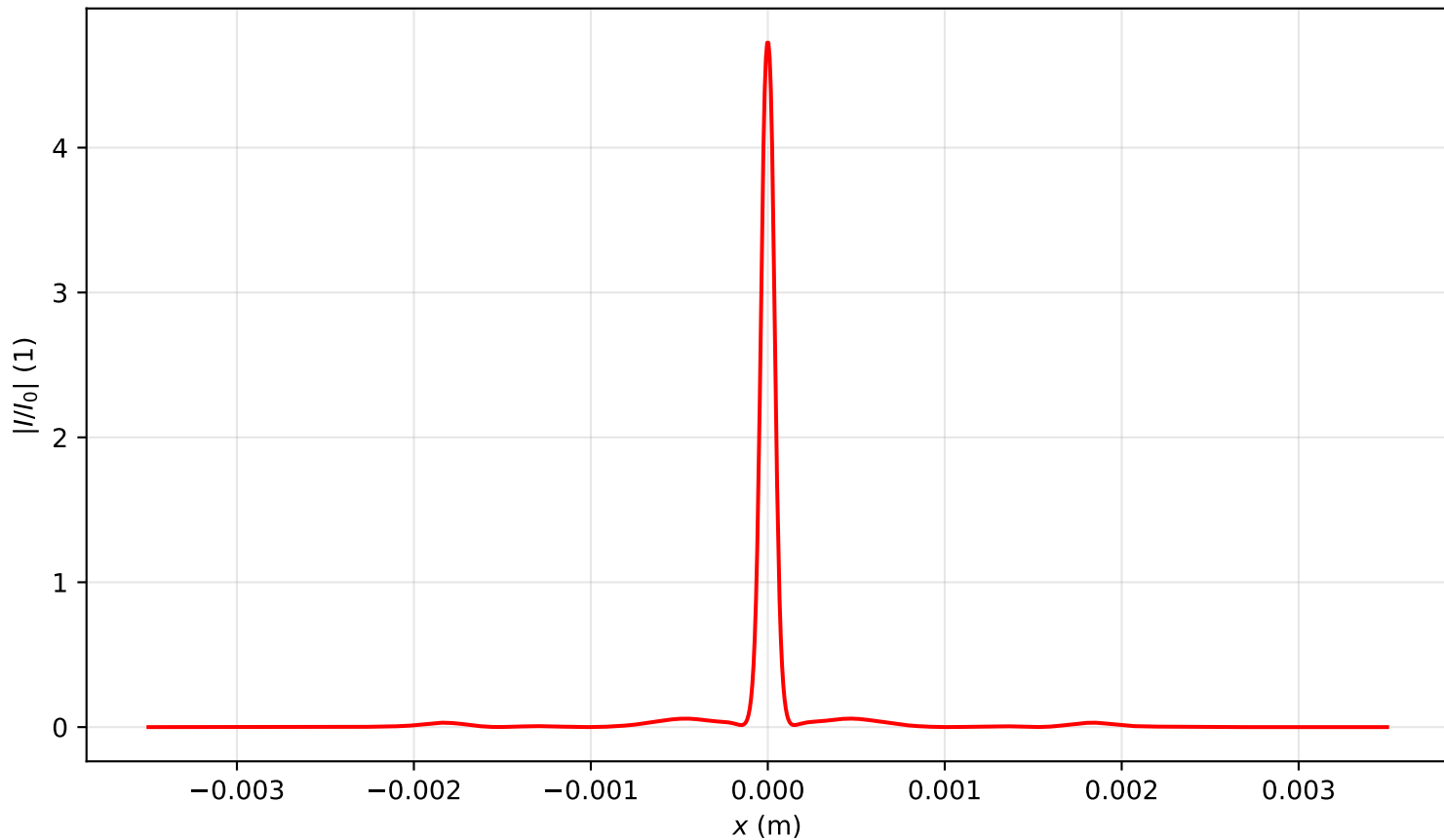
Intensity profile I(x, y = 0, z = 0.796)/I_0 , P_{in}=14.0P_{cr} , artificial time
