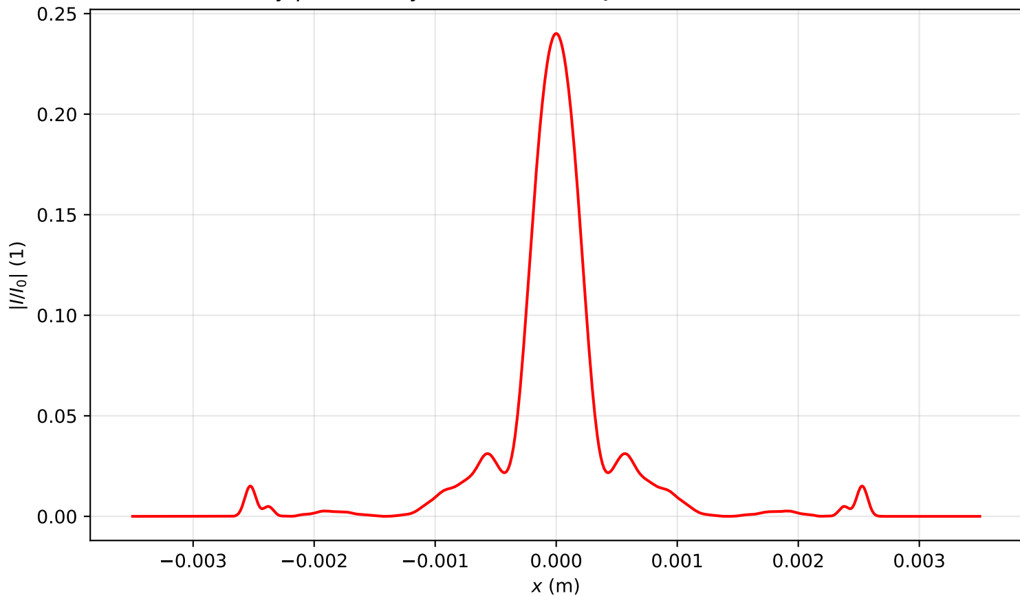
Intensity profile I(x, y = 0, z = 1.115)/I_0 , P_{in}=14.0P_{cr} , artificial time
