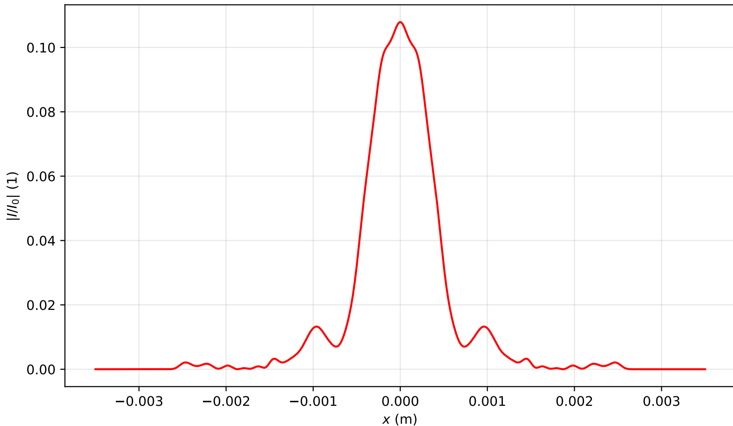
Intensity profile I(x, y = 0, z = 1.433)/I_0 , P_{in}=14.0P_{cr} , artificial time
