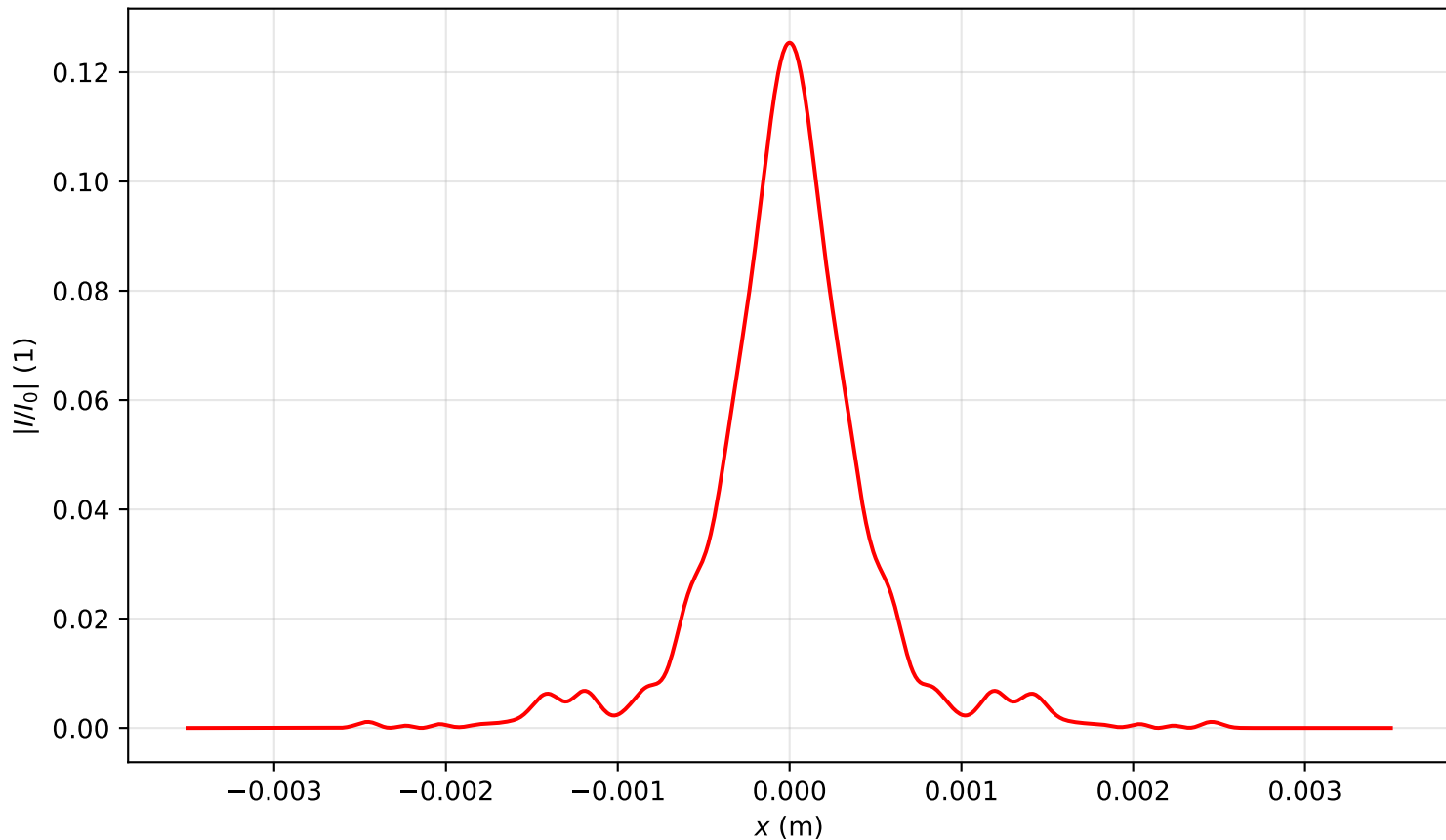
Intensity profile I(x, y = 0, z = 1.751)/I_0 , P_{in}=14.0P_{cr} , artificial time
