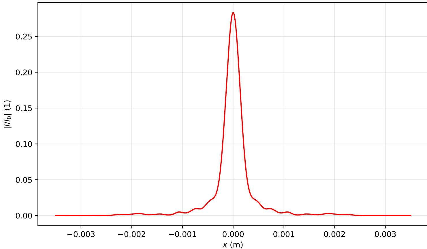
Intensity profile I(x, y = 0, z = 2.388)/I_0 , P_{in}=14.0P_{cr} , artificial time
