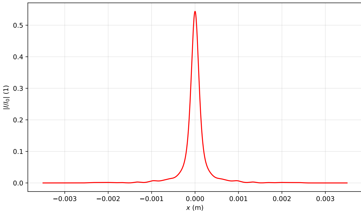
Intensity profile I(x, y = 0, z = 2.548)/I_0 , P_{in}=14.0P_{cr} , artificial time
