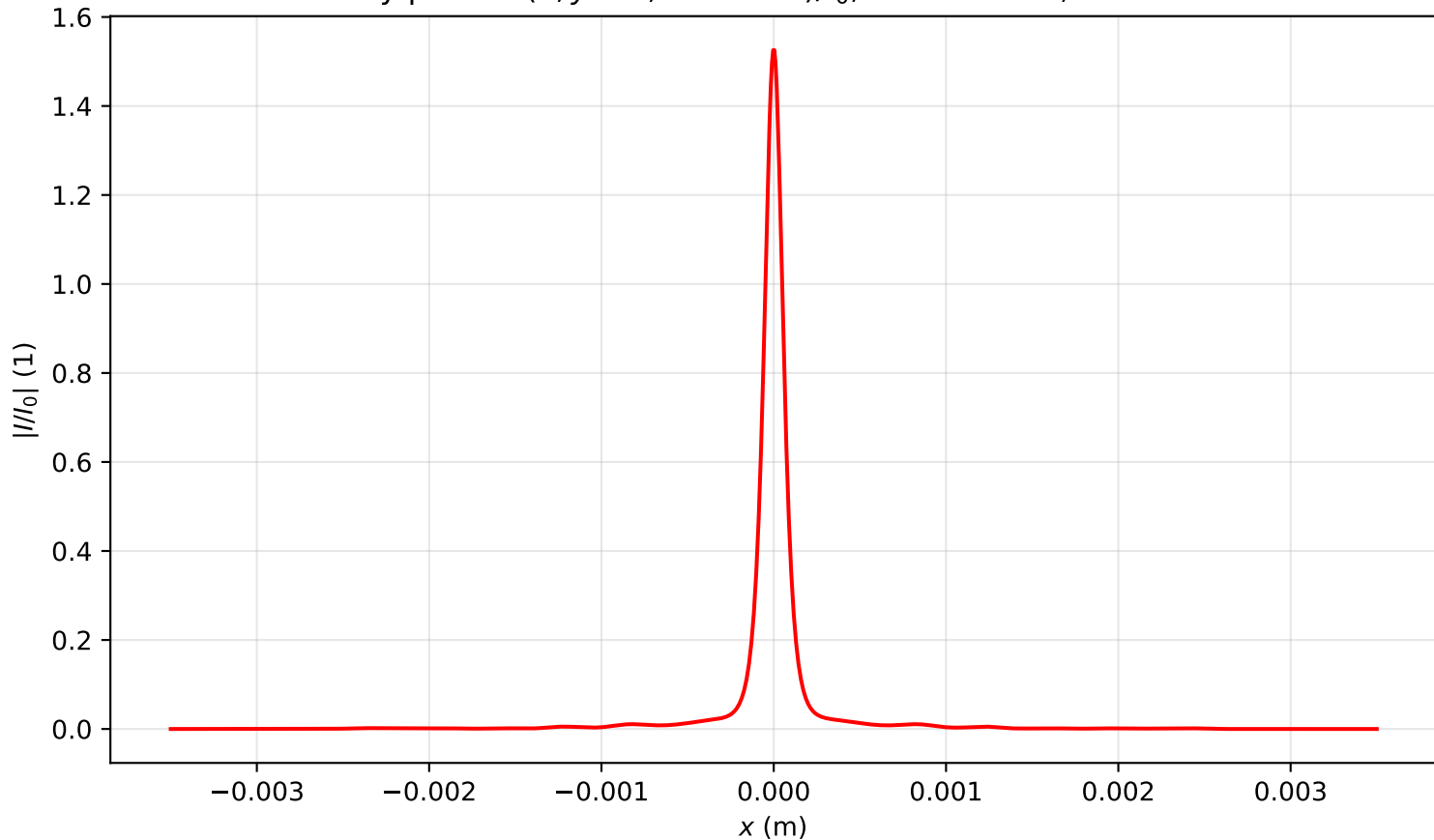
Intensity profile I(x, y = 0, z = 2.707)/I_0 , P_{in}=14.0P_{cr} , artificial time
