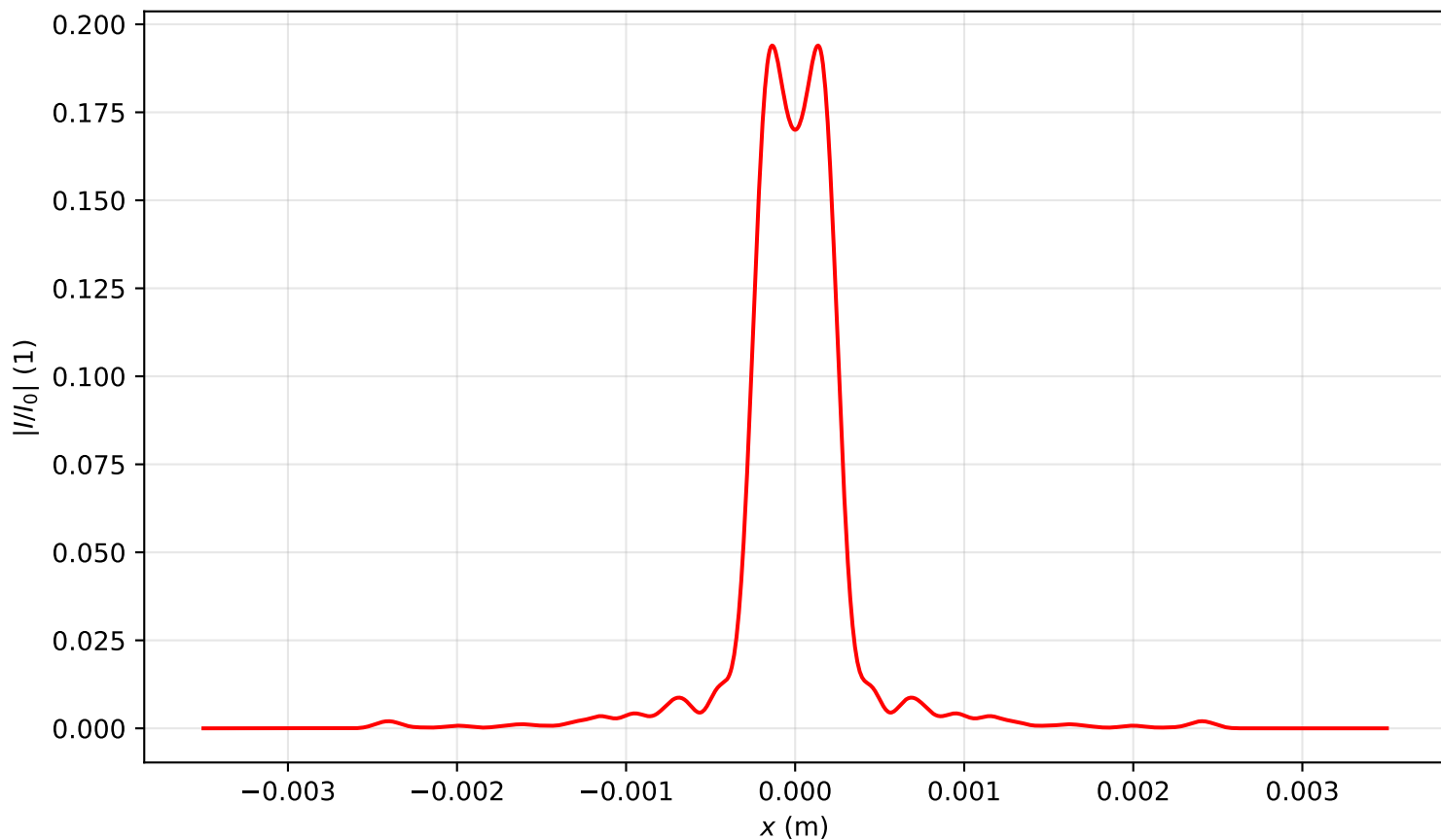
Intensity profile I(x, y = 0, z = 3.025)/I_0 , P_{in}=14.0\text{Pcr} , artificial time
