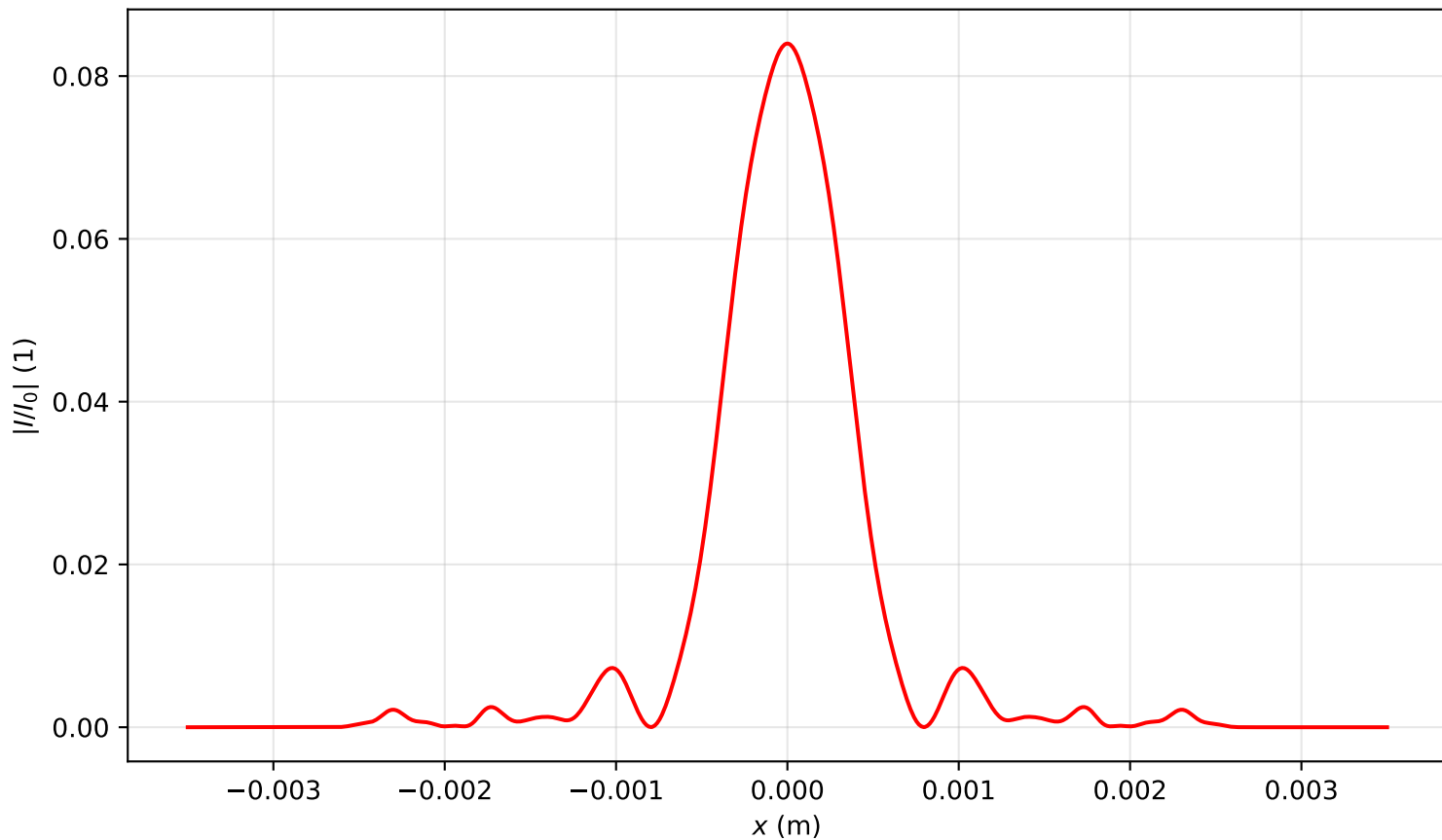
Intensity profile I(x, y = 0, z = 3.503)/I_0 , P_{in}=14.0\text{Pcr} , artificial time
