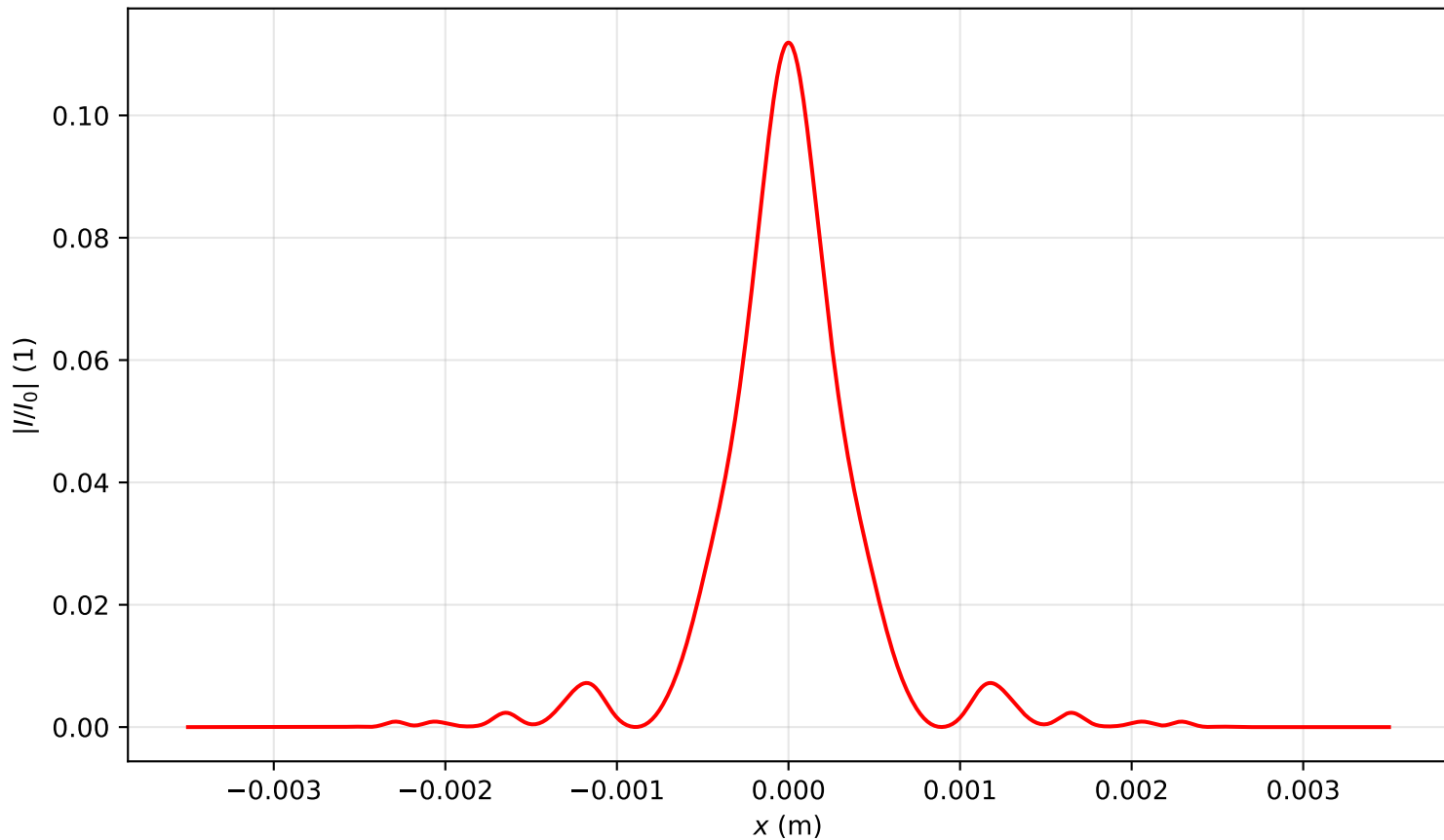
Intensity profile I(x, y = 0, z = 3.662)/I_0 , P_{in}=14.0P_{cr} , artificial time
