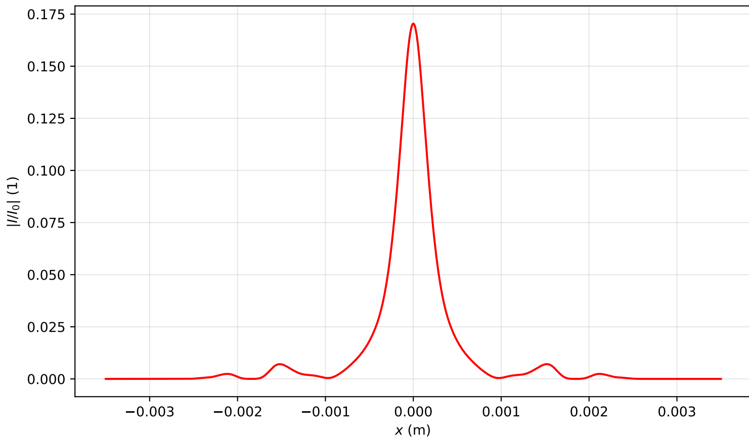
Intensity profile I(x, y = 0, z = 3.981)/I_0 , P_{in}=14.0P_{cr} , artificial time
