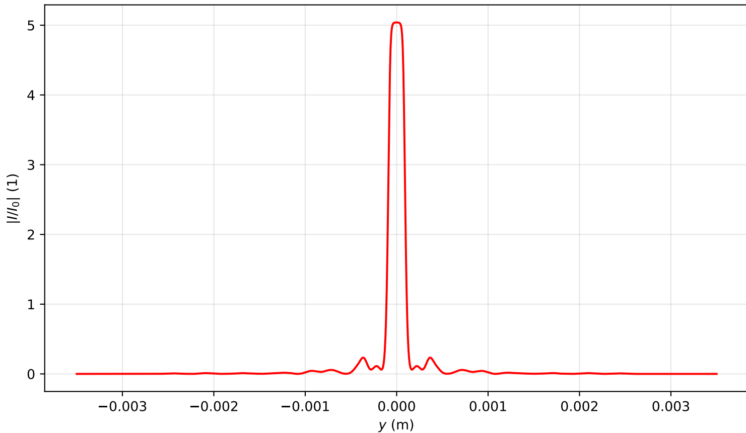
Intensity profile I(x=0, y, z=0.318)/I_0 , P_{in}=14.0P_{cr} , artificial time
