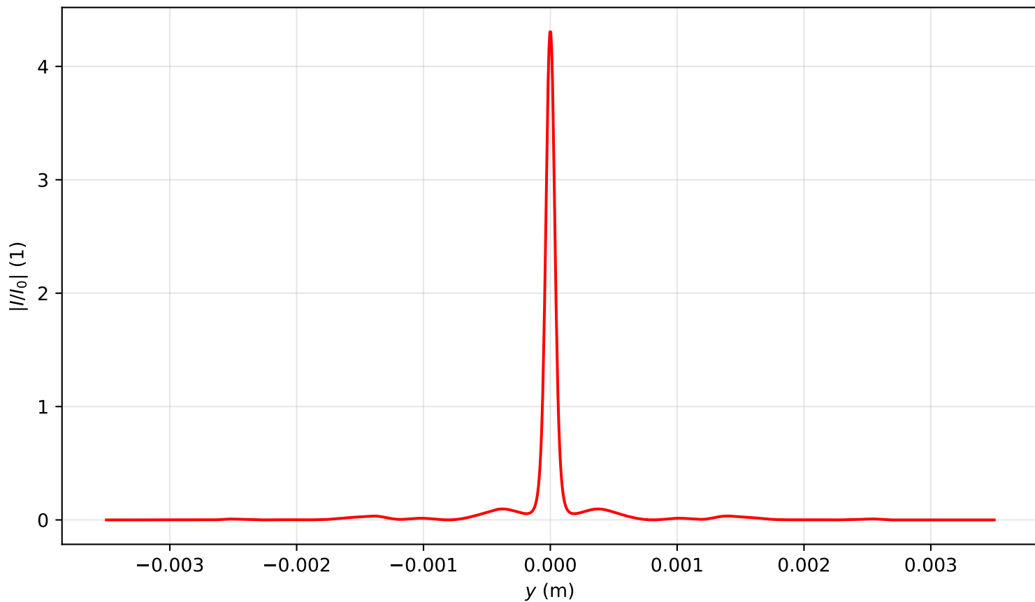
Intensity profile I(x=0, y, z=0.637)/I_0 , P_{in}=14.0P_{cr} , artificial time
