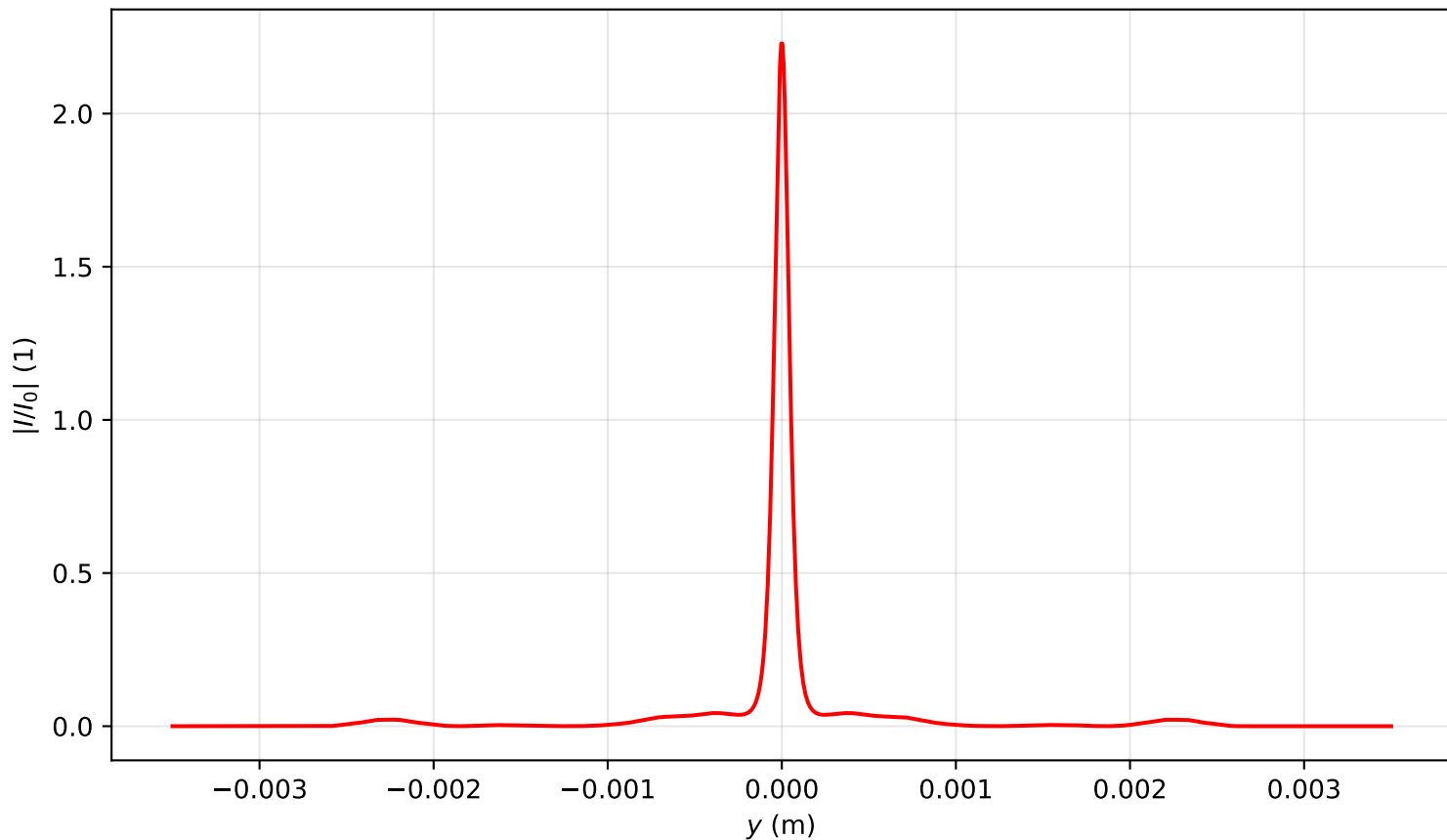
Intensity profile I(x=0, y, z=0.955)/I_0 , P_{in}=14.0P_{cr} , artificial time
