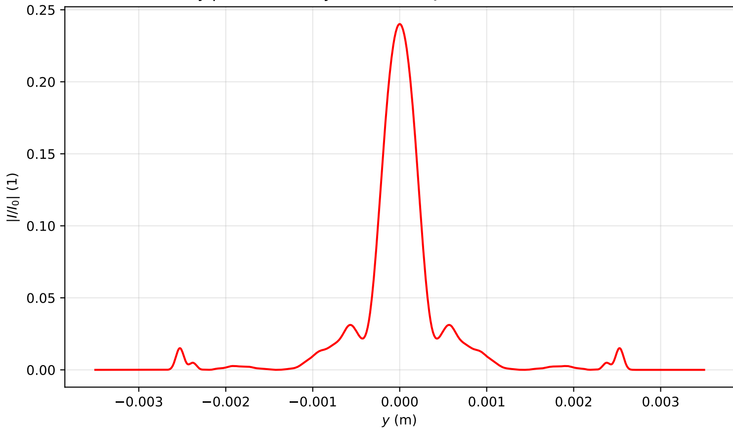
Intensity profile I(x=0, y, z=1.115)/I_0 , P_{in}=14.0P_{cr} , artificial time
