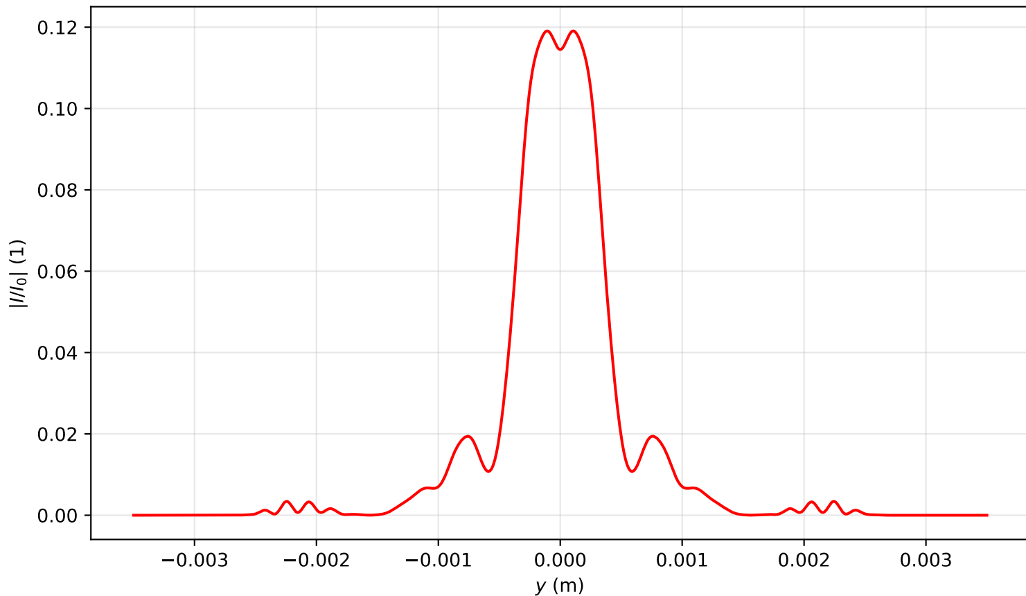
Intensity profile I(x=0, y, z=1.274)/I_0 , P_{in}=14.0\text{Pcr} , artificial time
