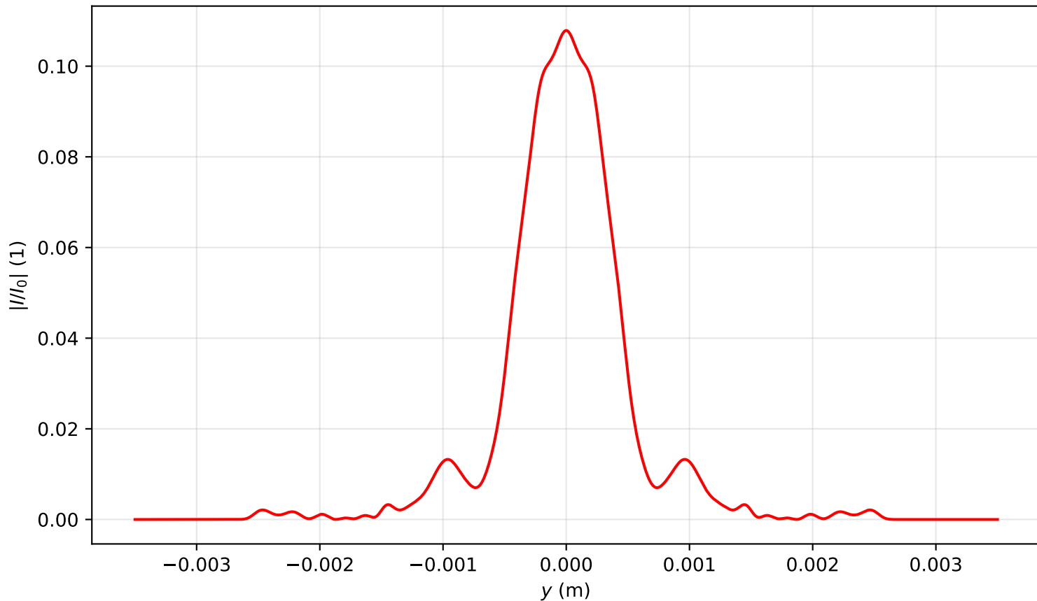
Intensity profile I(x = 0, y, z = 1.433)/I_0 , P_{in}=14.0P_{cr} , artificial time
