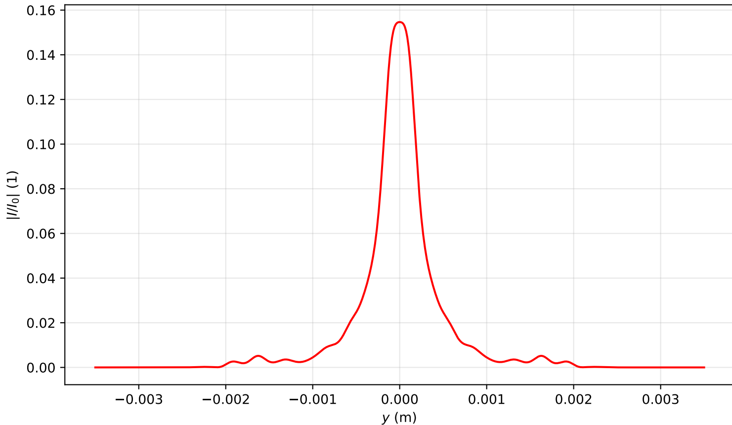
Intensity profile I(x = 0, y, z = 2.070)/I_0 , P_{in}=14.0\text{Pcr} , artificial time
