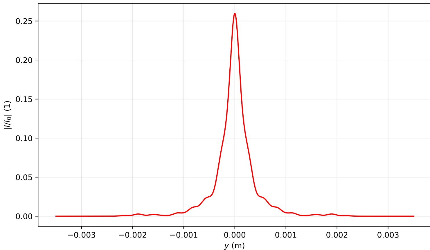
Intensity profile I(x=0, y, z=2.229)/I_0 , P_{in}=14.0P_{cr} , artificial time
