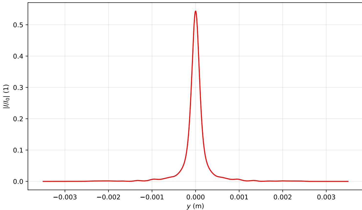
Intensity profile I(x=0, y, z=2.548)/I_0 , P_{in}=14.0P_{cr} , artificial time
