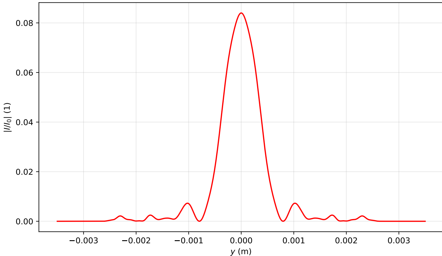
Intensity profile I(x = 0, y, z = 3.503)/I_0 , P_{in}=14.0\text{Pcr} , artificial time
