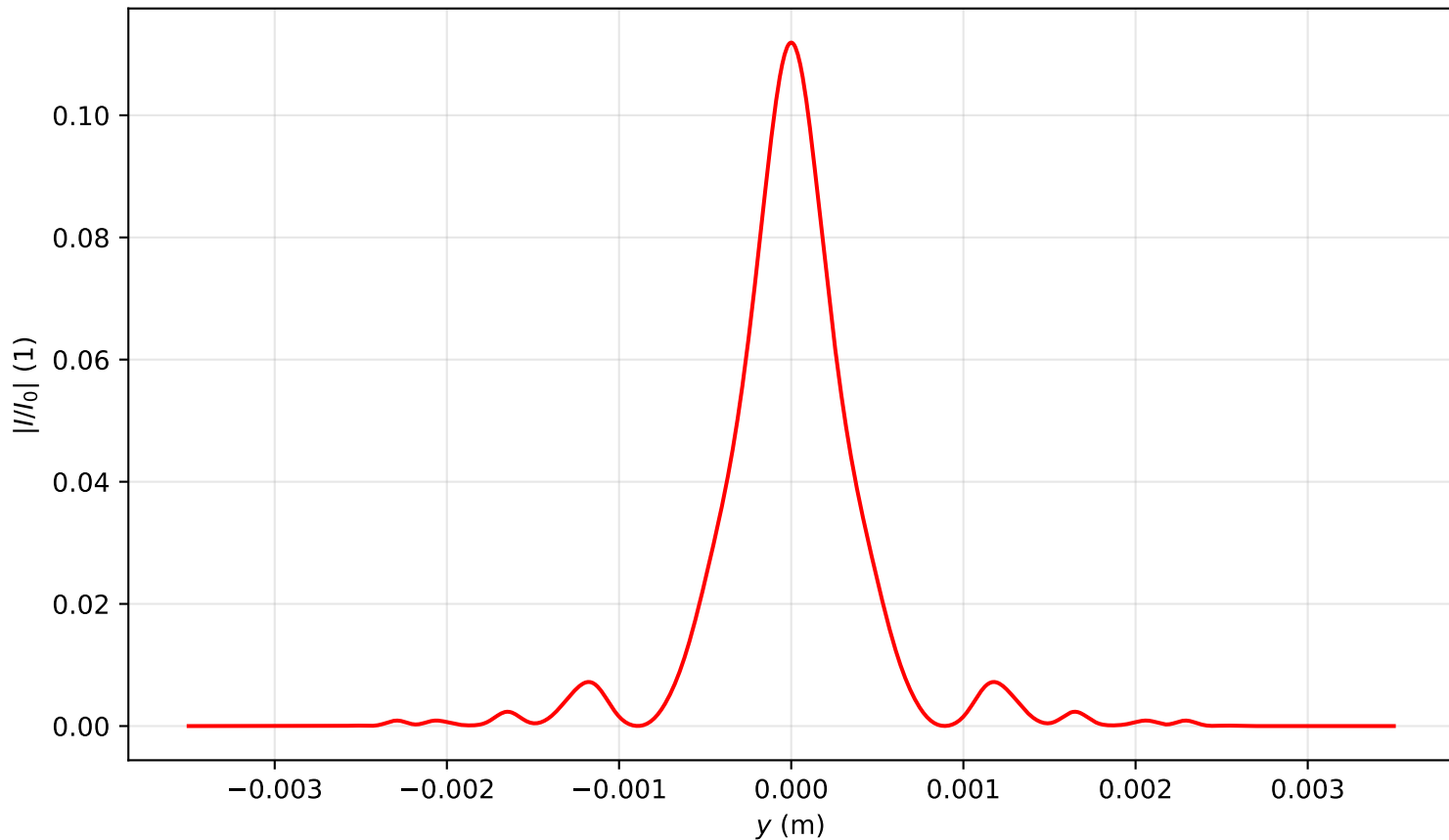
Intensity profile I(x = 0, y, z = 3.662)/I_0 , P_{in}=14.0P_{cr} , artificial time
