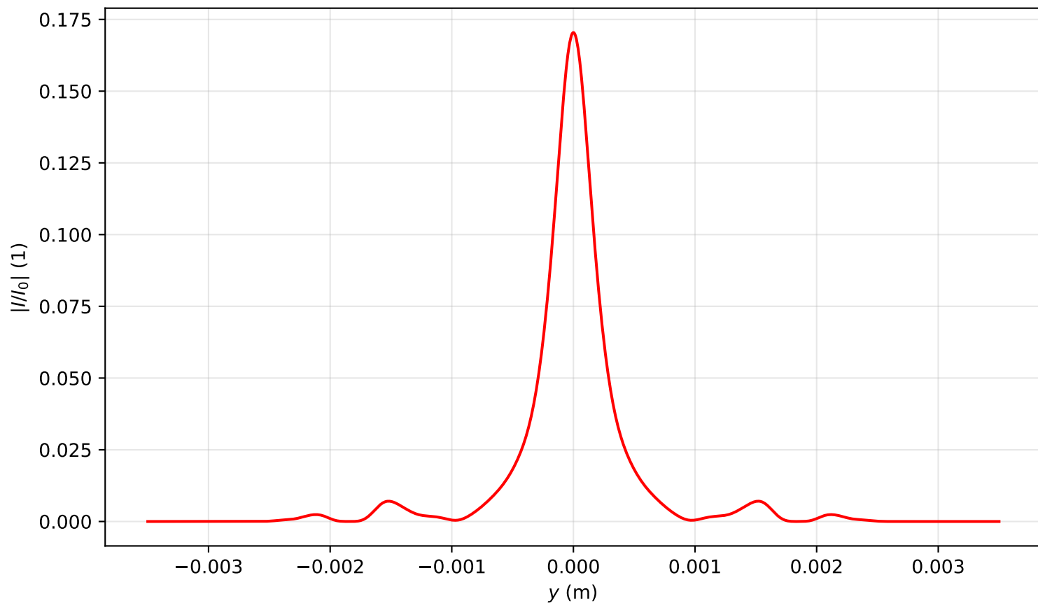
Intensity profile I(x=0, y, z=3.981)/I_0 , P_{in}=14.0P_{cr} , artificial time
