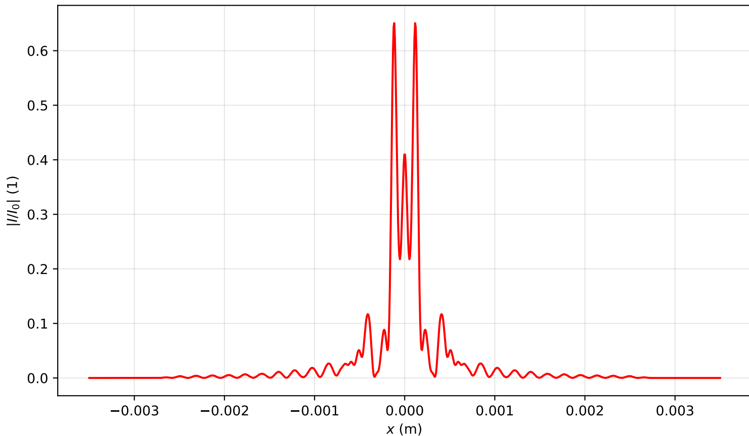
Intensity profile I(x, y = 0, z = 0.159)/I_0 , P_{in}=15.0P_{cr} , artificial time
