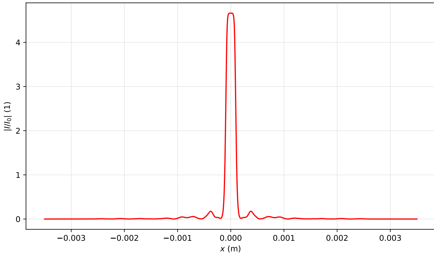
Intensity profile I(x, y = 0, z = 0.318)/I_0 , P_{in}=15.0P_{cr} , artificial time
