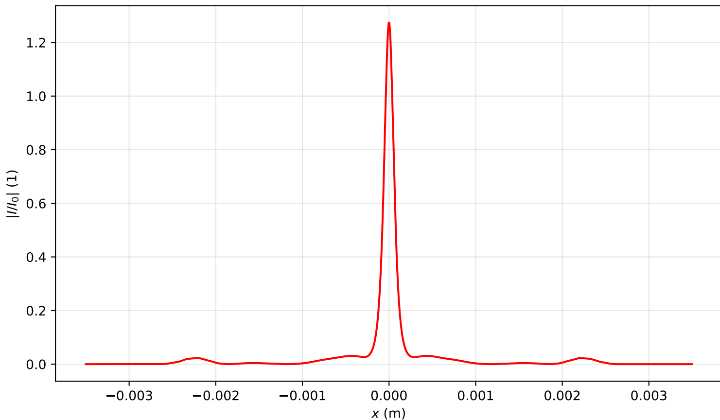
Intensity profile I(x, y = 0, z = 0.955)/I_0 , P_{in}=15.0P_{cr} , artificial time
