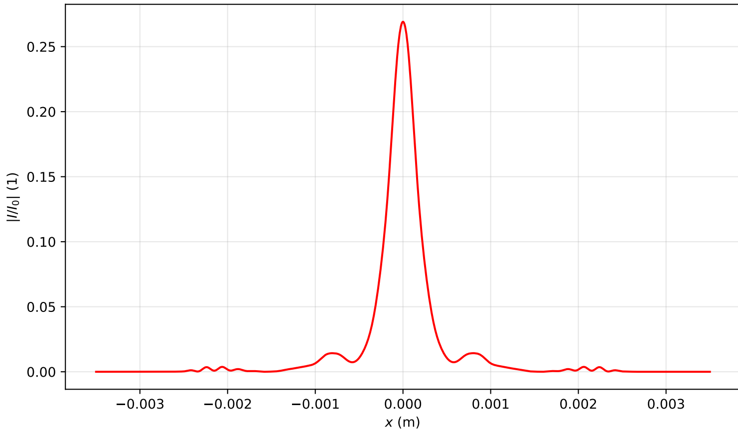
Intensity profile I(x, y = 0, z = 1.274)/I_0 , P_{in}=15.0P_{cr} , artificial time
