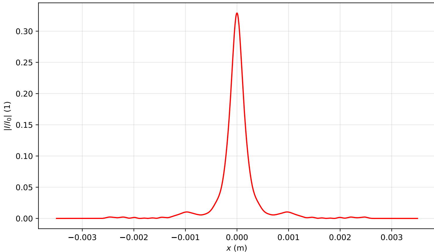
Intensity profile I(x, y = 0, z = 1.433)/I_0 , P_{in}=15.0P_{cr} , artificial time
